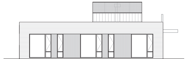
East elevation
